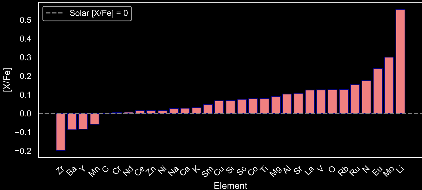
Abundance Pattern for GALAH Star Field [70] (N=315)
