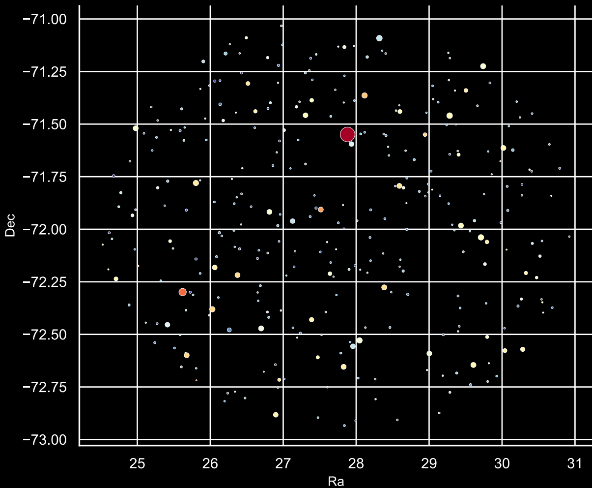
Field [70] Ra [27.69] Dec [-71.95] Stars: 315
