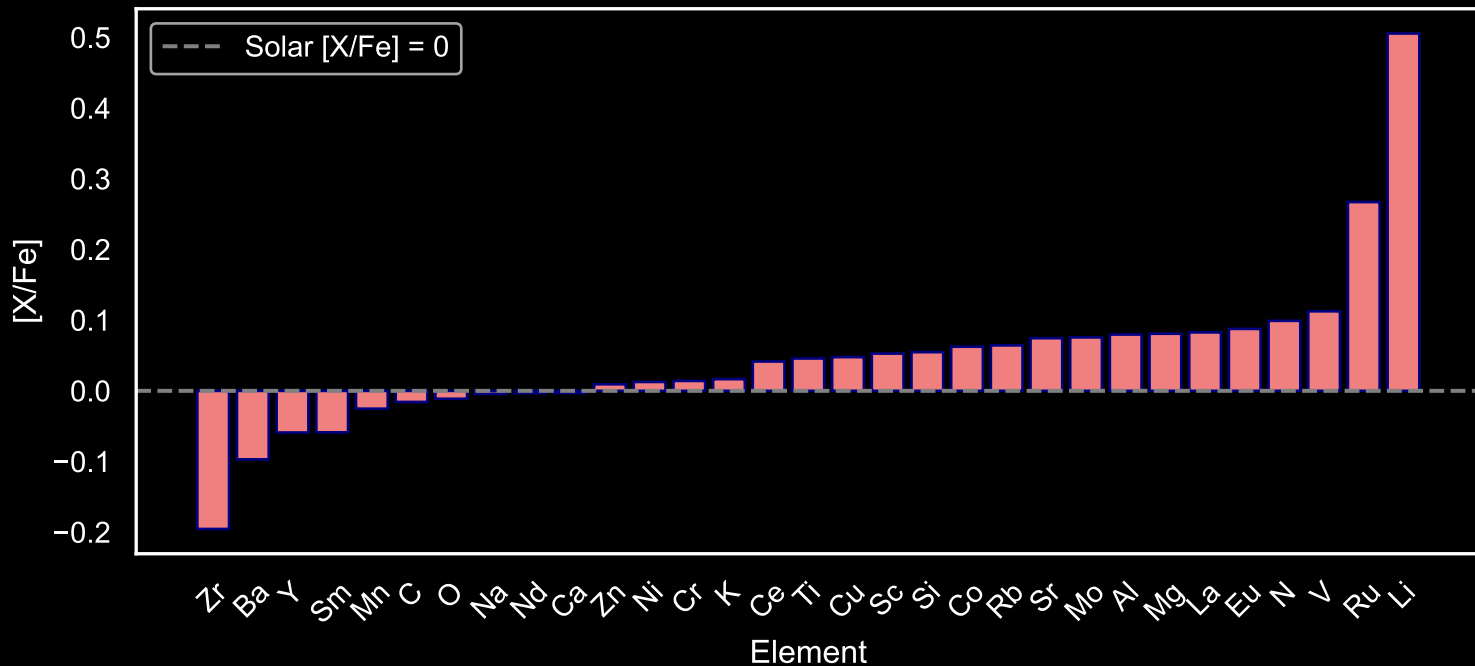
Abundance Pattern for GALAH Main Sequence Stars: Star Field [70] (N=152)
