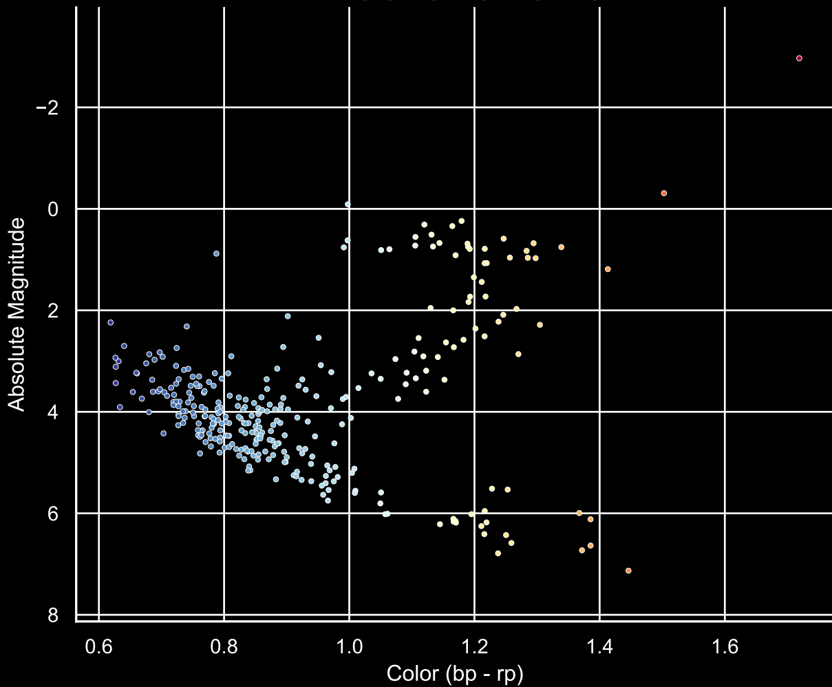
GALAH Hertzprung-Russel Diagram Field [70] Ra [27.69] Dec [-71.95]
