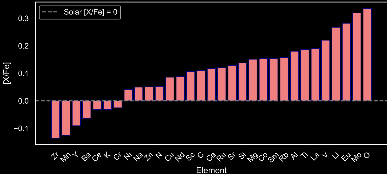
Abundance Pattern for GALAH Red Giants: Star Field [70] (N=58)
