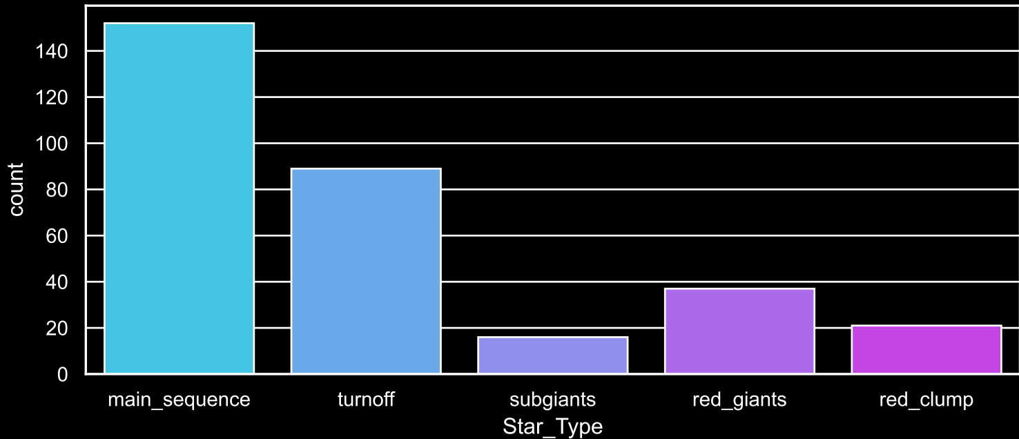
Field [70] Count plot of Star Type
